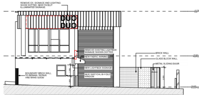
03 SIDE ELEVATION 1:100
