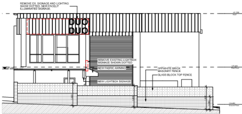
01 CHAPEL ST ELEVATION 1:100
