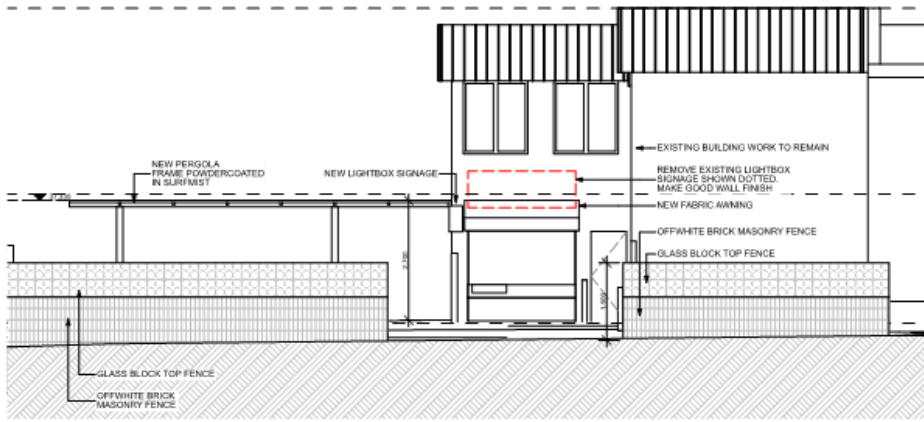
02 LESLIE ST ELEVATION 1:100
